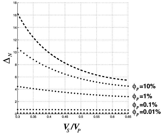
FIG. 2. Influence of equant porosity \phi_p on the normal weakness of a crack system connected to isometric pores (dotted lines). The dashed line (on top) shows the normal weakness for isolated dry cracks; \Delta_N = 0 corresponds to isolated fluid-filled cracks. The vertical scale is in the units of crack density e . The parameters of the crack system are the aspect ratio \alpha = 0.0005 , the volume portion occupied by the cracks \phi_c = 0.01\% , and the crack density e = 0.05 . The cracks are filled with water that has the bulk modulus k' = 2 GPa. The P -wave velocity in the host rock is V_P = 5 km/s.
